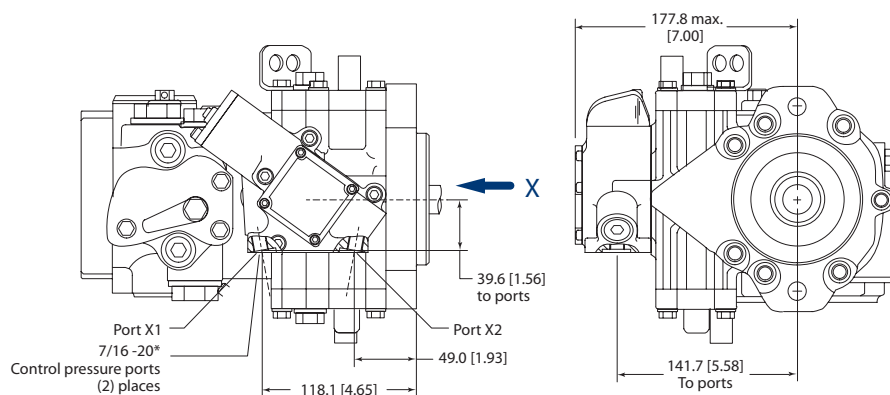
Side view Variable pump with HDC
