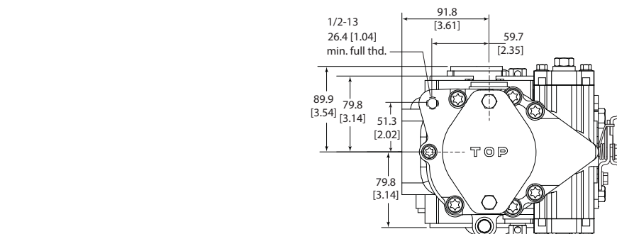
No auxiliary mounting flange
