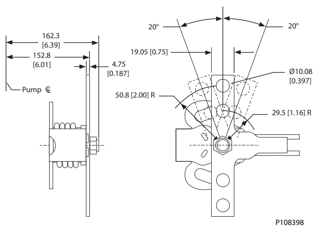
Control handle with heavy spring and heavy duty four hole handle
