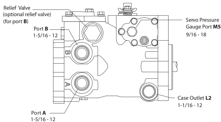
Bottom view (with MDC and suction filtration)
