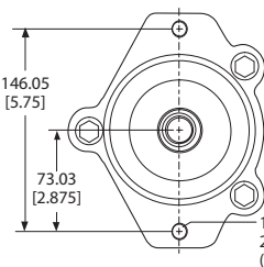
SAE B Auxiliary mounting flange Option B
