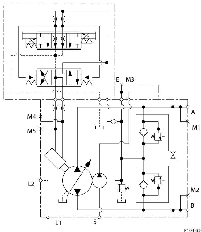
EDC Hydraulic Schematic
